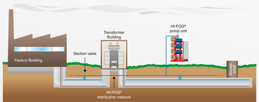
An example of a HI-FOG® system for cable tunnels
